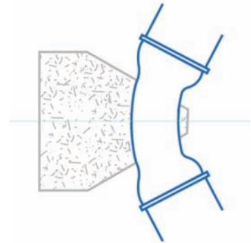
Anchoring at points of change of direction
