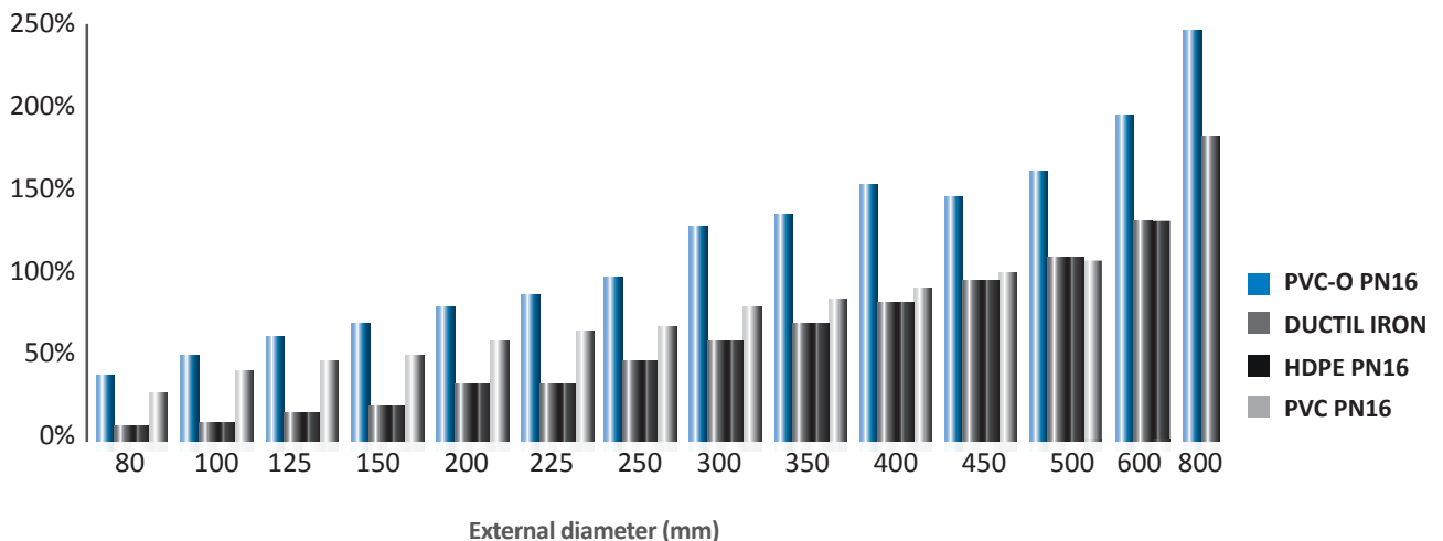
Hydraulic capacity/Piping costs compared to TOM® PVC-O PN16 DN250
