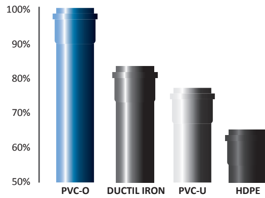
Hydraulic capacity
